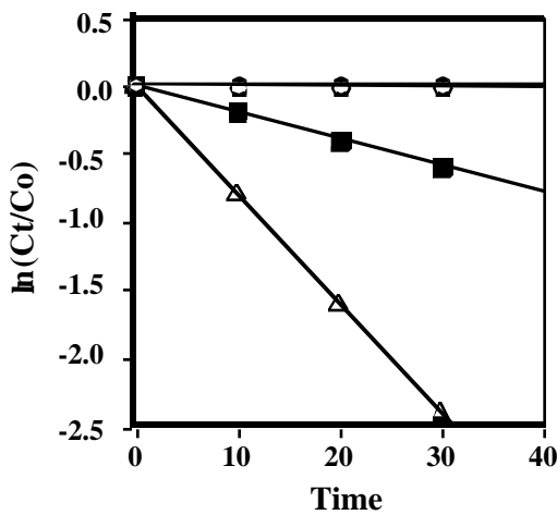
Figure 5. Activity assay for exchange activity of Ats1p. Assays were carried out as described in the text. Results are plotted as rates of exchange of GTP for [ 3 H]GDP on Ran in the presence of buffer (O) or 50 fmol 6-His-Prp20p (△) or 6-His-Ats1p (■).
